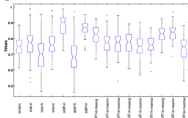
Figure 5. APFD Distributions for Siemens Programs.
